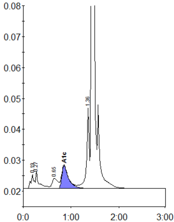
Peak table - ID: 10805603
