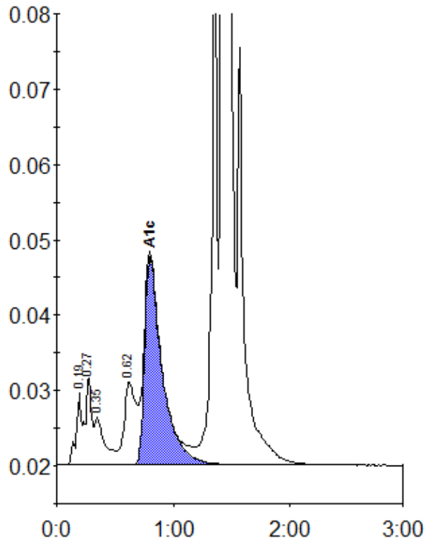
Peak table - ID: 10743287
