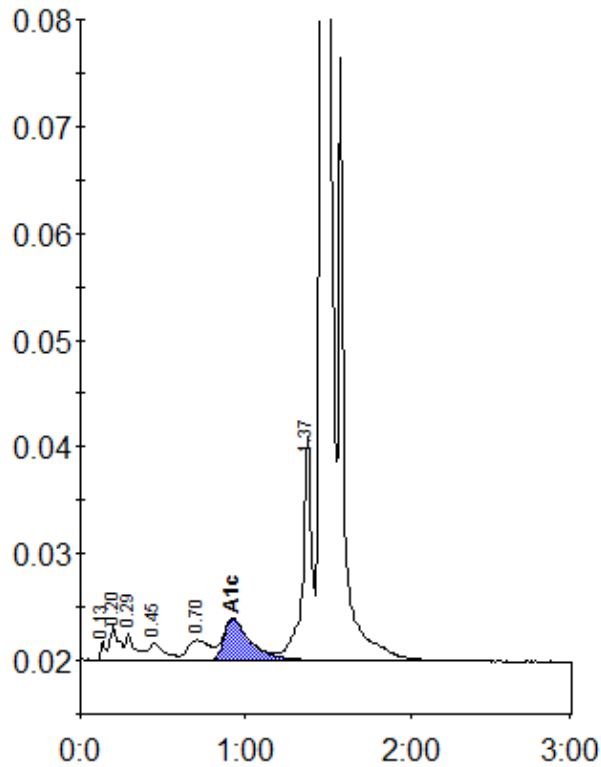
Peak table - ID: 10855323
