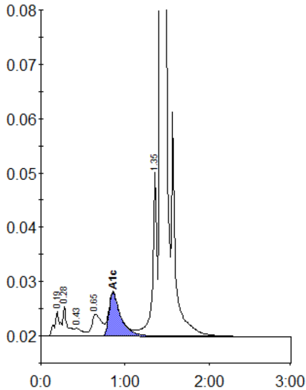
Peak table - ID: 10867481
