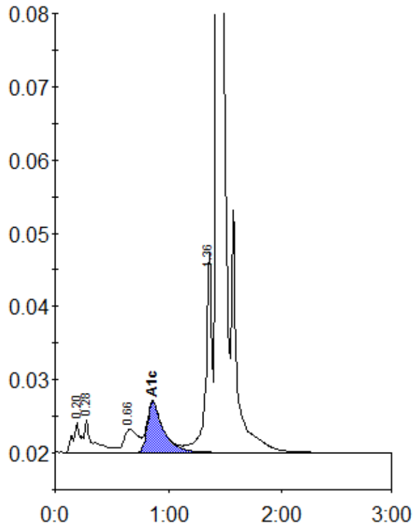
Peak table - ID: 10840601
