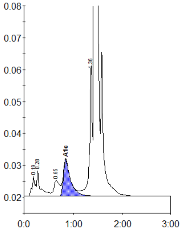
Peak table - ID: 10866655
