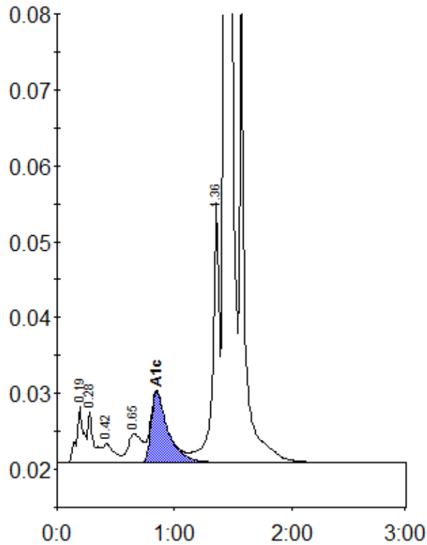
Peak table - ID: 10814829
