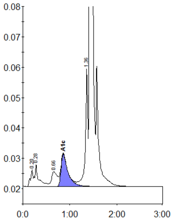
Peak table - ID: 10840724
