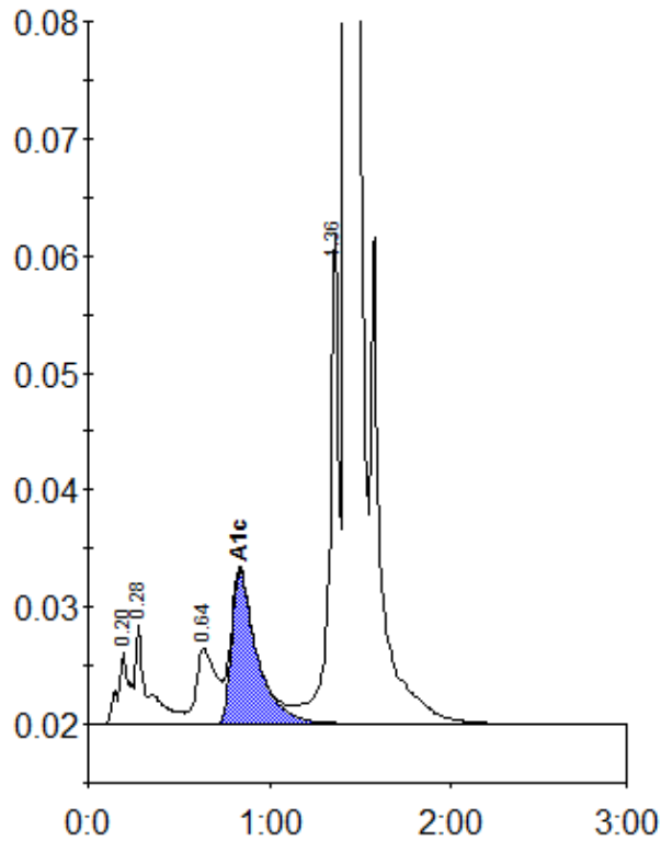
Peak table - ID: 10840722
