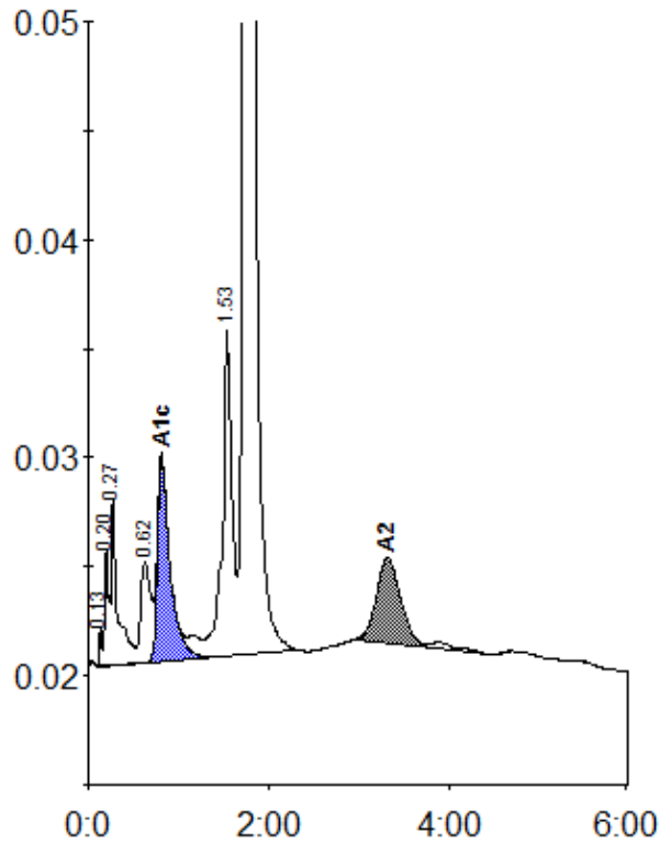
Peak table - ID: 10884489
