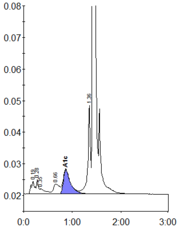
Peak table - ID: 10836915
