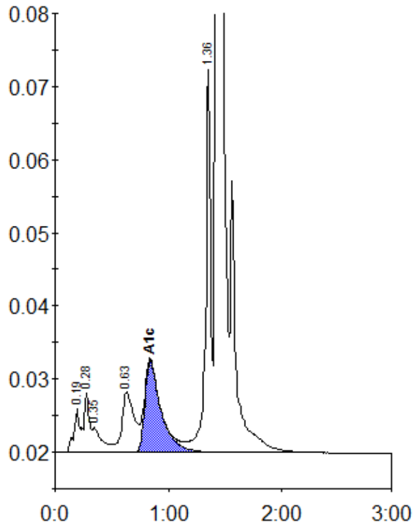
Peak table - ID: 10866972
