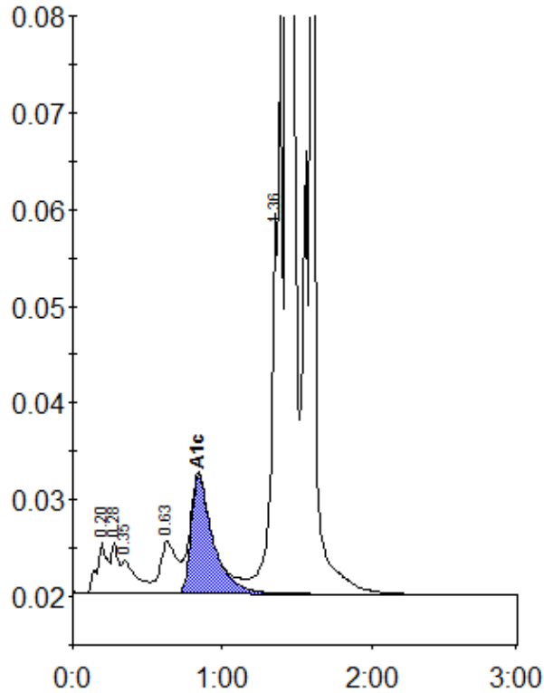
Peak table - ID: 10884065
