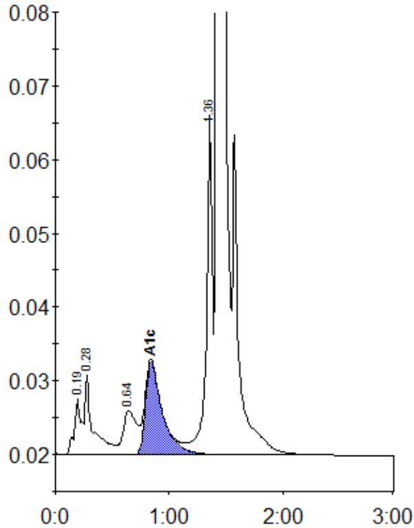
Peak table - ID: 10867774
