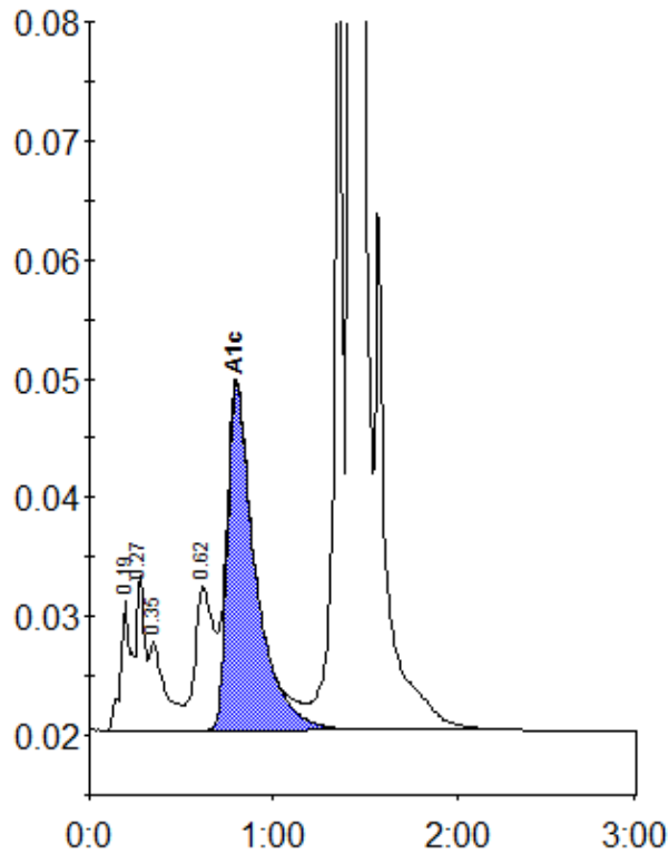
Peak table - ID: 10867448
