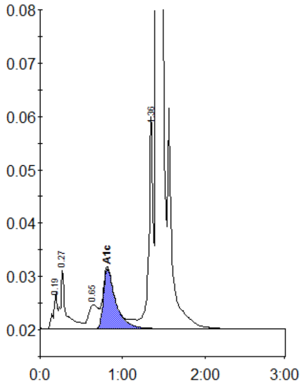
Peak table - ID: 10652264
