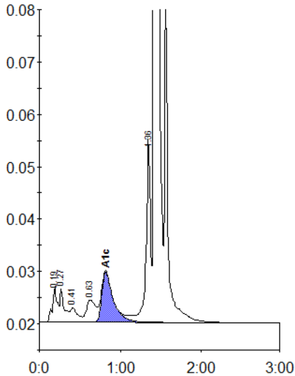
Peak table - ID: 10855868
