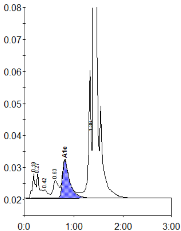
Peak table - ID: 10792250
