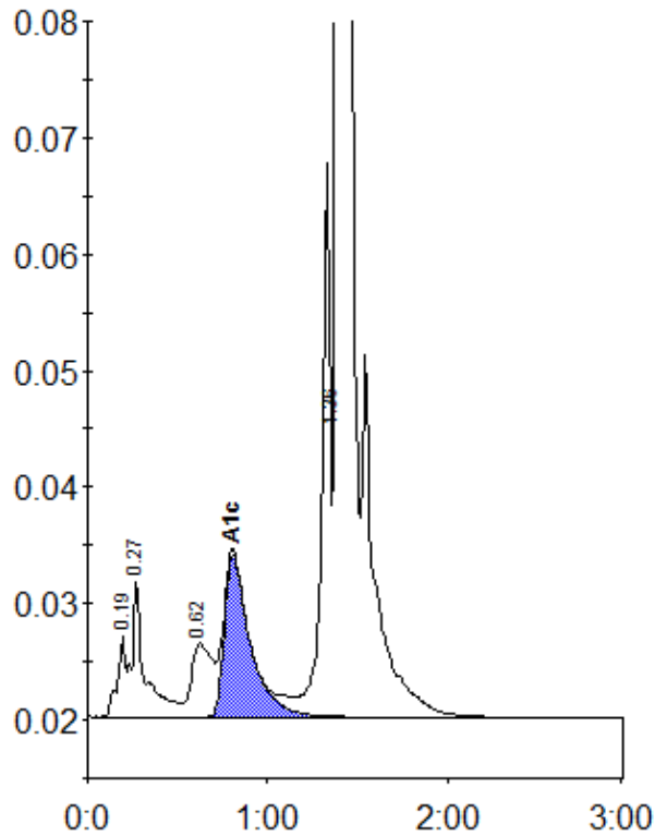
Peak table - ID: 10788669
