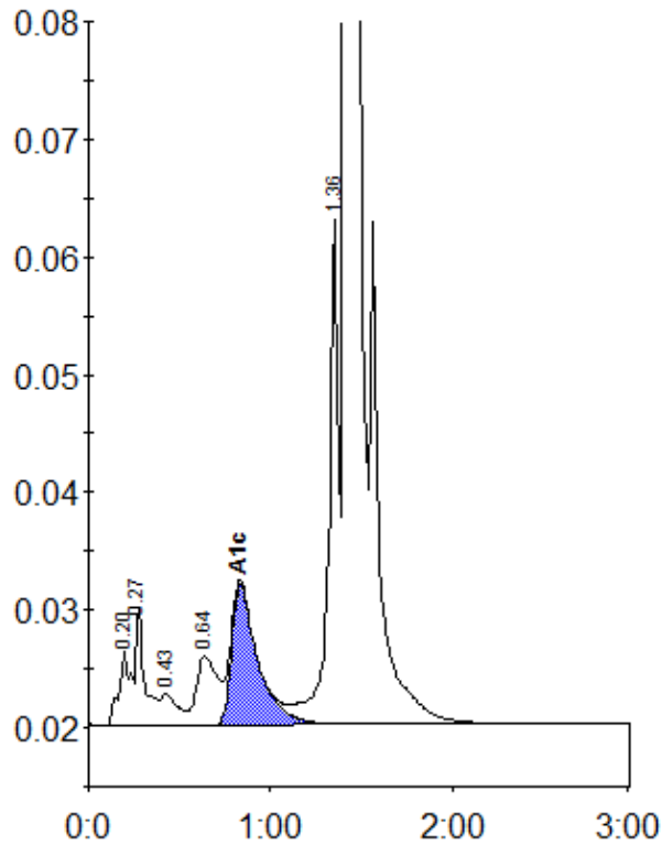
Peak table - ID: 10800359
