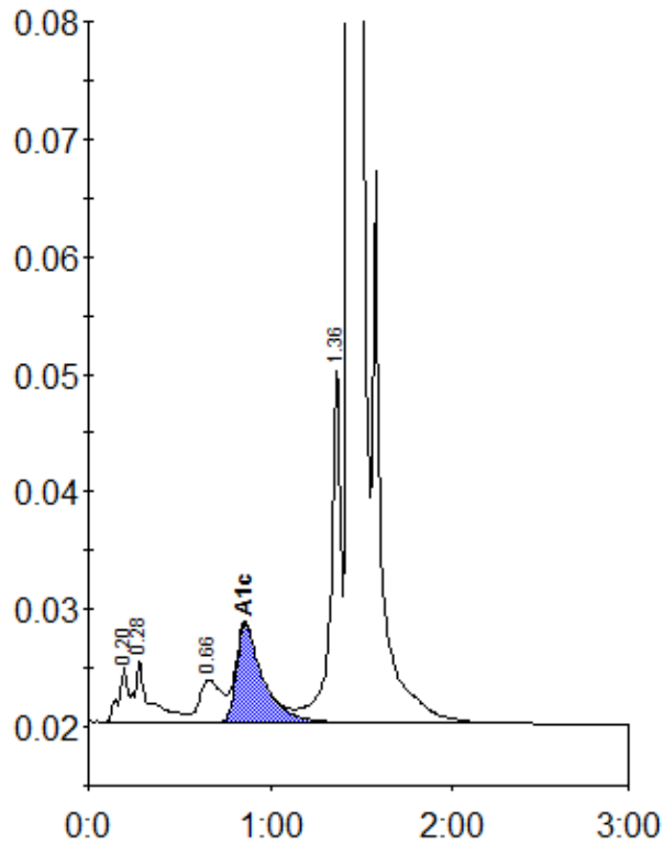
Peak table - ID: 10822578
