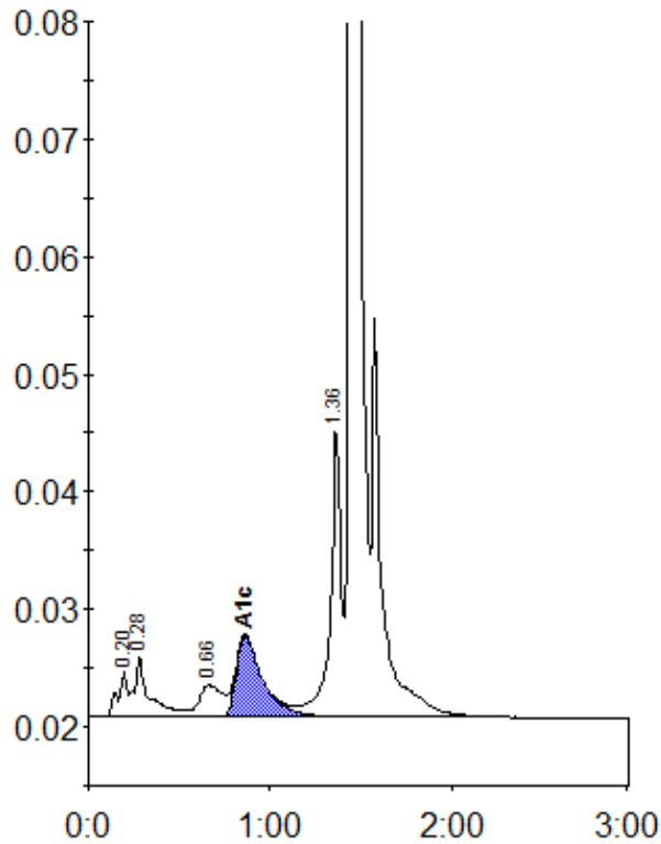
Peak table - ID: 10814605
