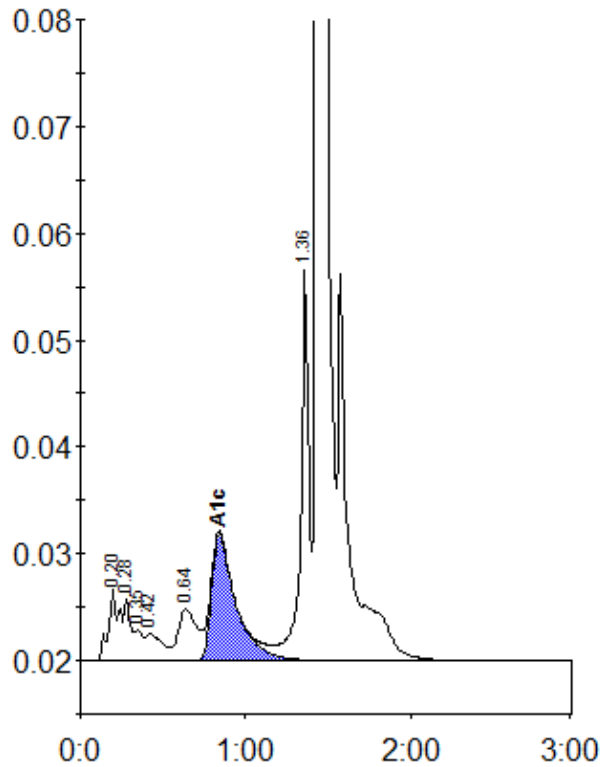
Peak table - ID: 10701857
