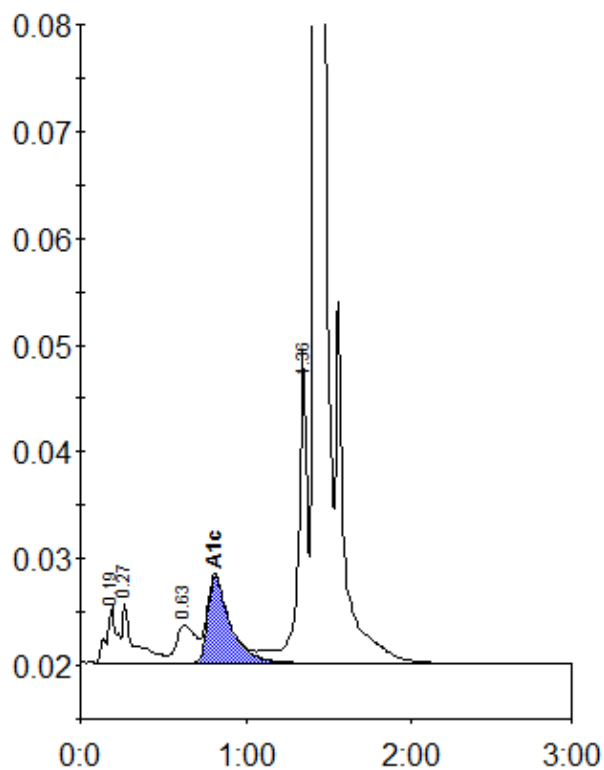
Peak table - ID: 10821923
