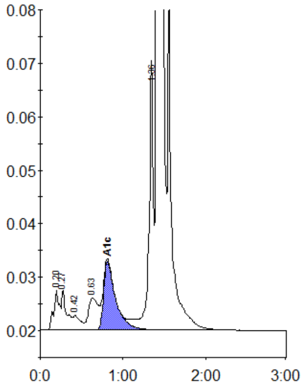
Peak table - ID: 10756497
