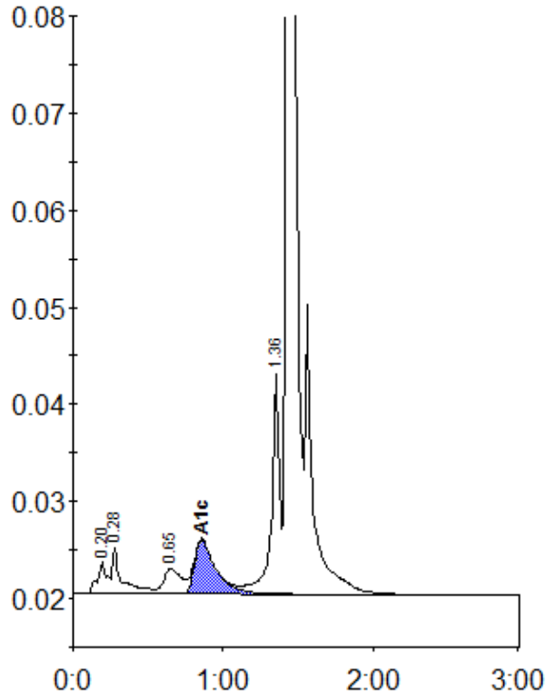
Peak table - ID: 10811662
