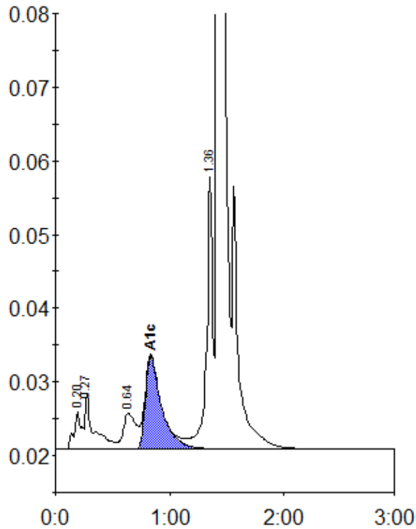
Peak table - ID: 10778428
