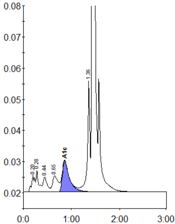
Peak table - ID: 10825272
