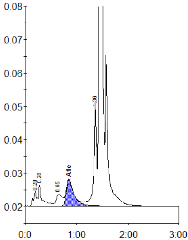
Peak table - ID: 10825300
