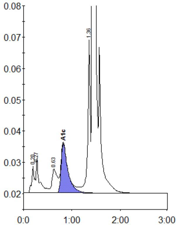
Peak table - ID: 10826029
