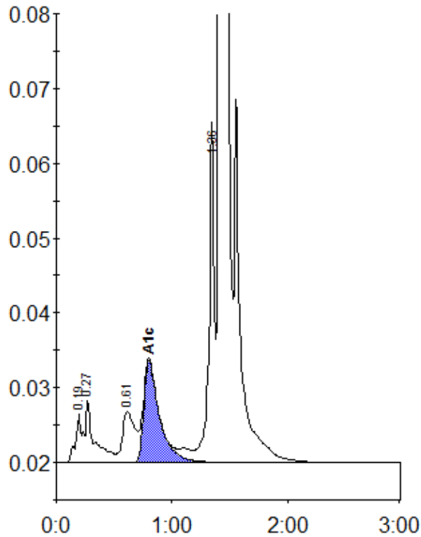
Peak table - ID: 10747173
