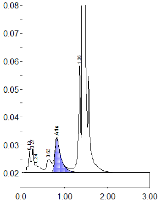
Peak table - ID: 10606816
