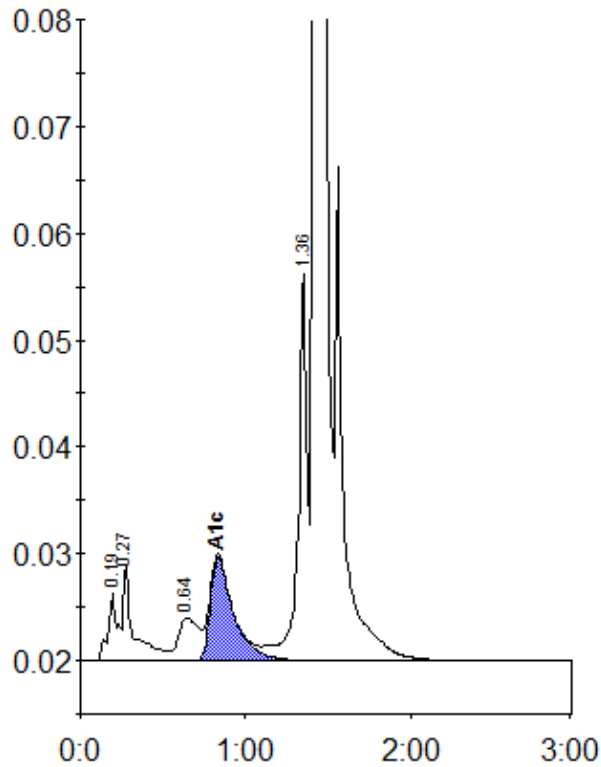
Peak table - ID: 10819262
