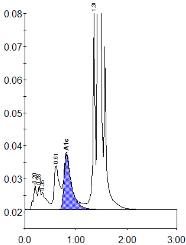
Peak table - ID: 10758434
