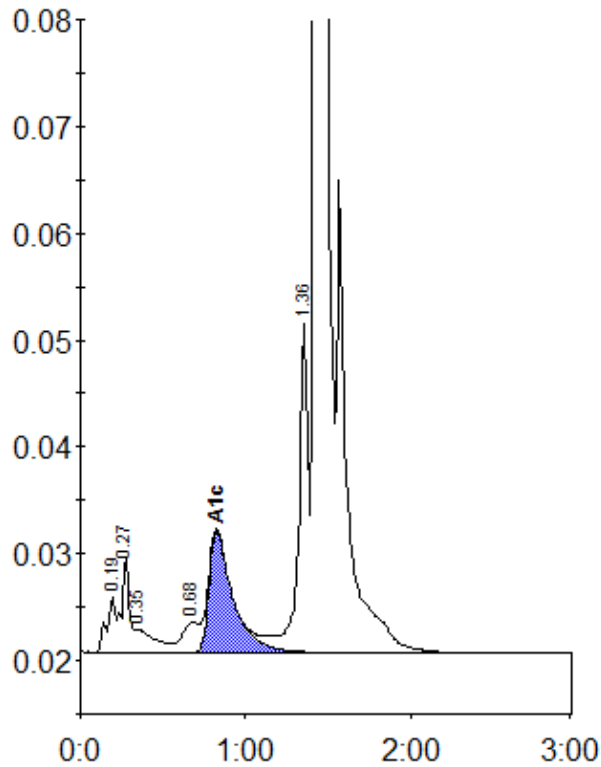
Peak table - ID: 10770851
