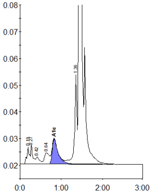
Peak table - ID: 10828772
