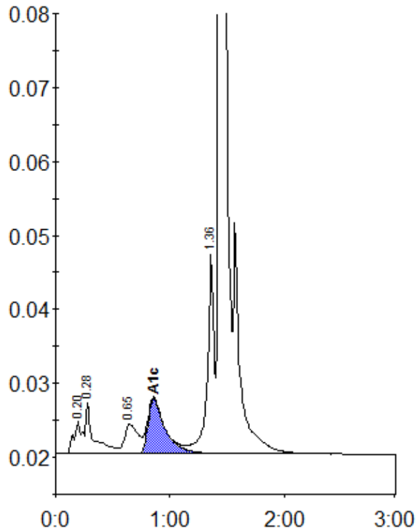
Peak table - ID: 10819037
