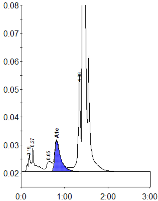
Peak table - ID: 10819548
