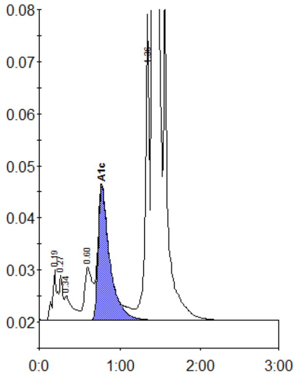
Peak table - ID: 10744005
