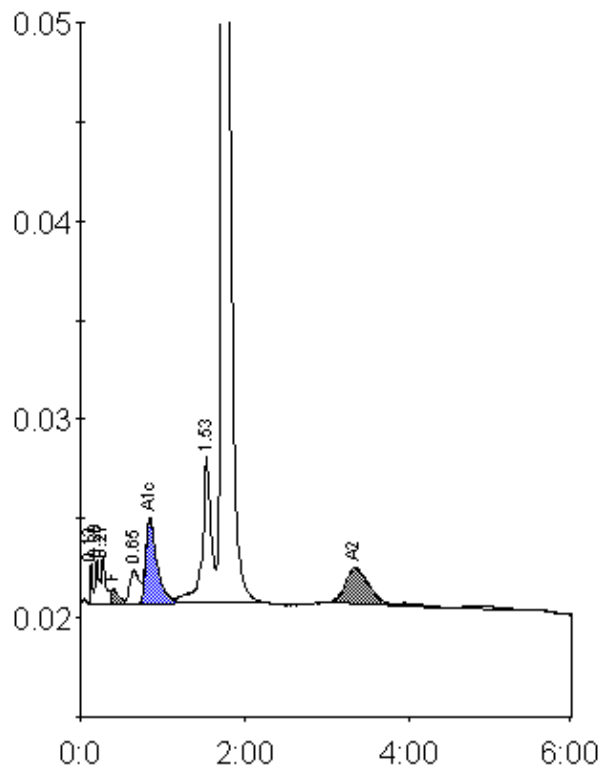
Peak table - ID: 10825951
