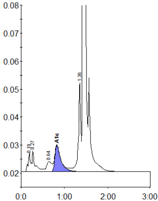
Peak table - ID: 10761149
