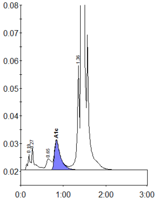
Peak table - ID: 10538852
