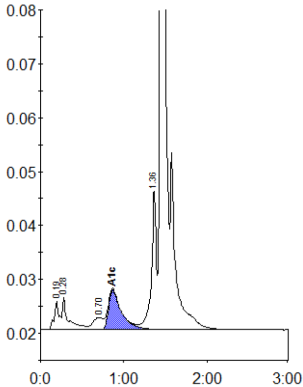
Peak table - ID: 10653007
