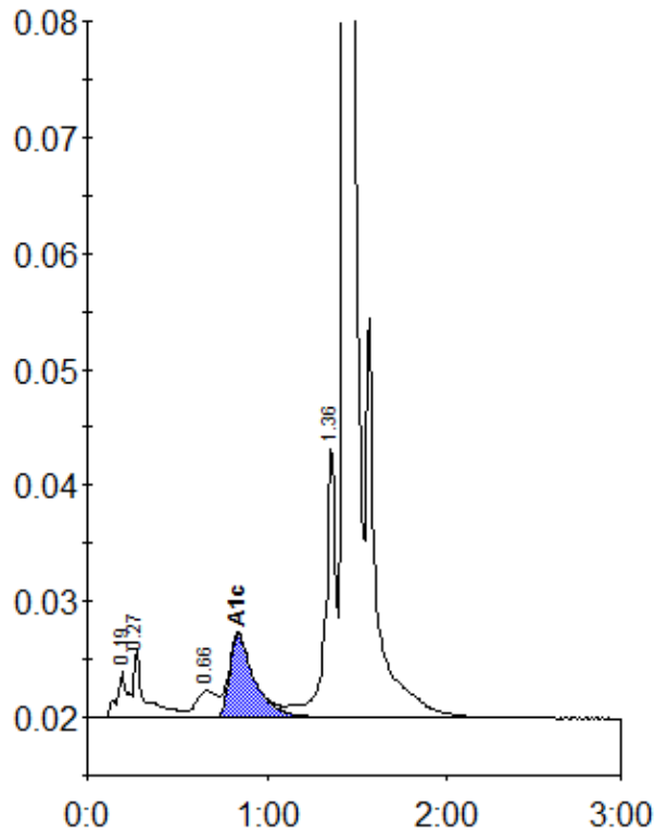
Peak table - ID: 10497819
