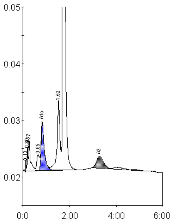
Peak table - ID: 10746868
