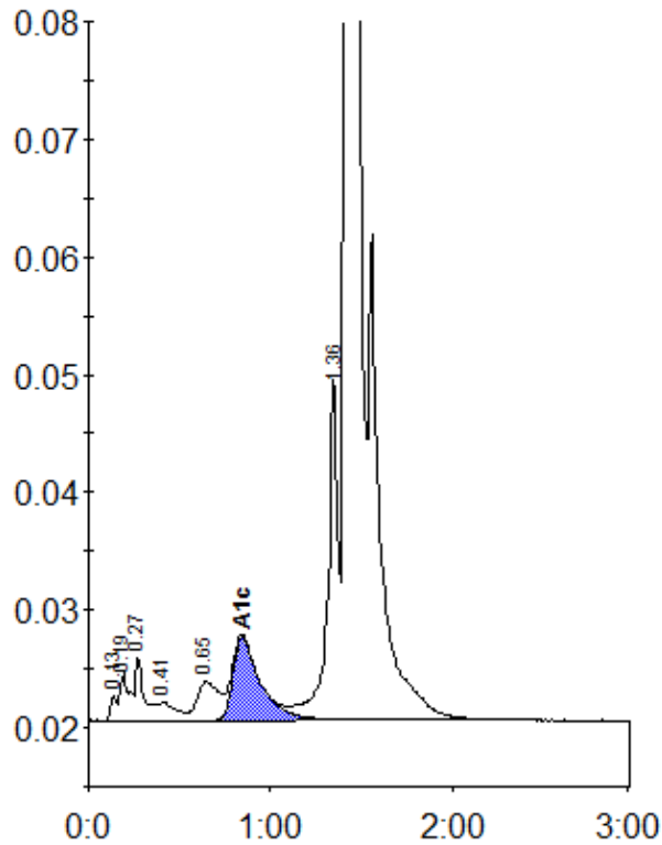
Peak table - ID: 10754154
