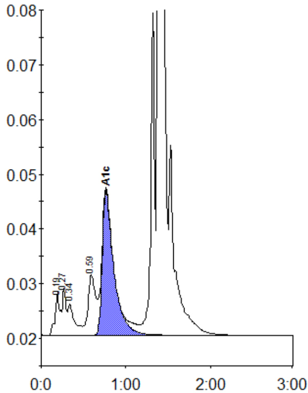
Peak table - ID: 10772641
