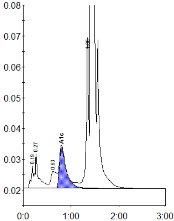
Peak table - ID: 10767356
