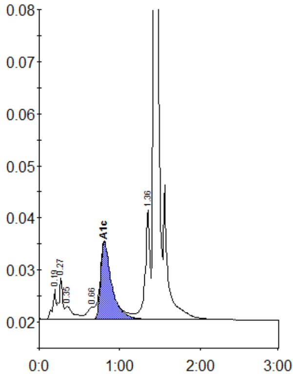
Peak table - ID: 10740526
