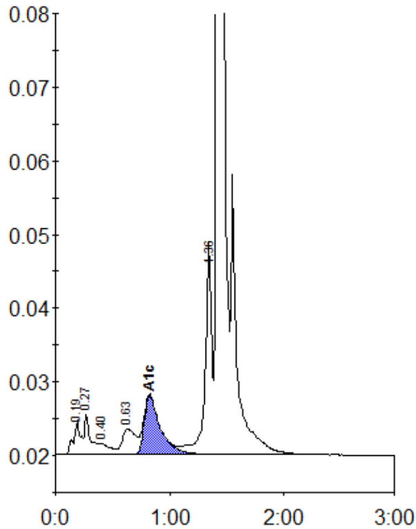
Peak table - ID: 10751657
